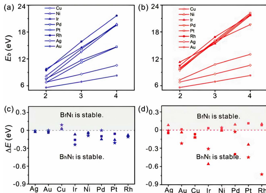
Fig. 3 Binding energies as a function of BN clusters terminated with (a) N and (b) B atoms. The difference in formation energy between B_nN_t and B_tN_t of (c) N and (d) B terminated BN clusters. Squares, stars, and triangles represent the cluster size of 2, 3, and 4, respectively. 180
