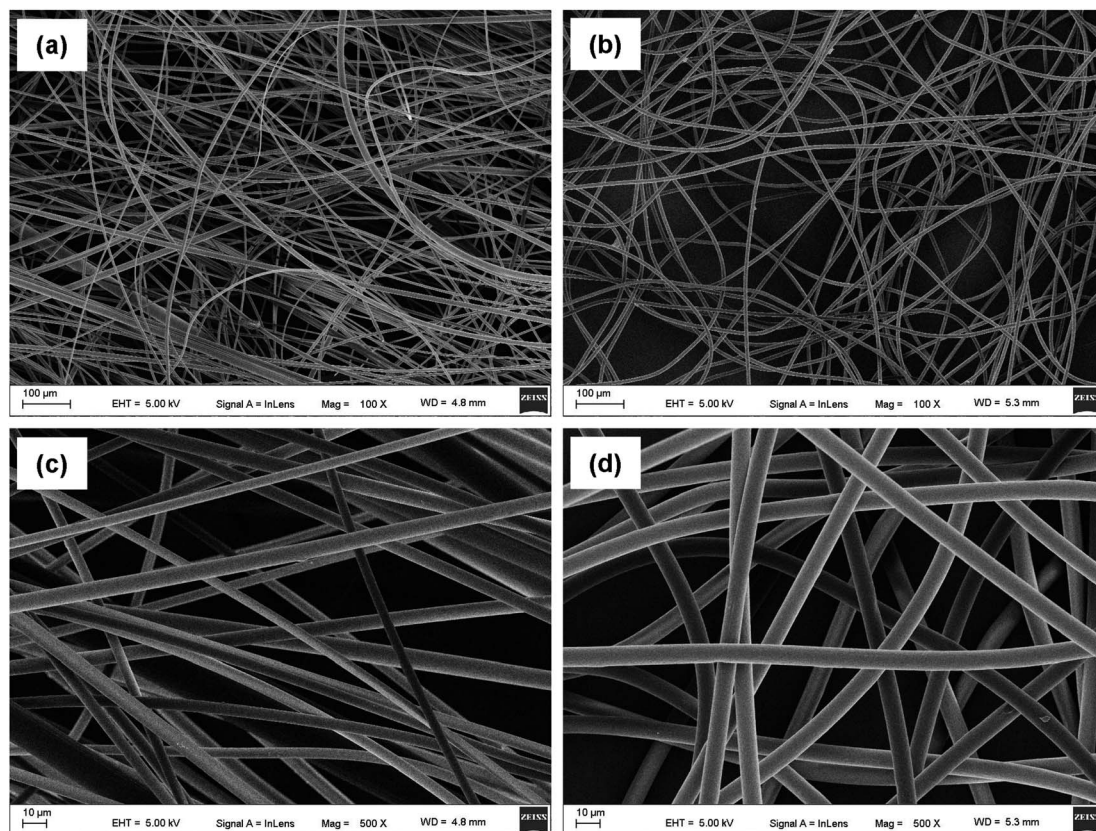
Fig. 2 SEM images of the PS-Eu 1 -Tb 60 fiber membrane (a and c) and the neat PS fiber membrane (b and d).
