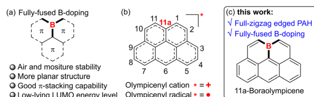
Fig. 1 (a) Illustration of fully-fused B-doping and potential unique properties. (b) Skeletal structures of carbon-based olympicenes. (c) Full-zigzag edged and fully-fused B-doped 11a-boraolympicene reported in this work.
