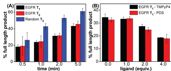
Fig. 10 Percentage of the full-length product obtained from Taq polymerase reactions. (A) Reactions performed using templates T 1 –T 3 at different time points. (B) Reactions performed using T 1 with increasing concentrations of ligands (TMPyP4 and PDS) at 2 min. For gel images, see Fig. S23B and S24.†
