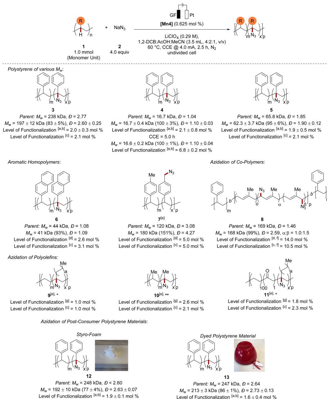
Scheme 1 Scope of the mangana-electrocatalyzed azidation. Standard reaction conditions: 1 (1.0 mmol, 1.0 equiv.), 2 (4.0 mmol, 4.0 equiv.), [Mn4] (6.25 \mu\text{mol} ), \text{LiClO}_4 (0.29 M), 1,2-DCB (2.0 mL), AcOH (1.0 mL), MeCN (0.5 mL), CCE @ 4.0 mA at 60^\circ \text{C} under \text{N}_2 for 2.5 h. The mass average molar mass and dispersity ( \bar{D} ) were determined by GPC against narrow-disperse polystyrene standards using THF as eluent at 30^\circ \text{C} and were reported as the molar weight retention of the parent polymer. *Reaction performed at 80^\circ \text{C} . **Reaction performed at 120^\circ \text{C} . a The level of functionalization was estimated using an IR- ^1\text{H} NMR correlation curve ( m = 2.7051 \text{ mol } \% , R^2 = 0.9942 ) and the relative IR intensity of the \text{N}_3 -band ( 2106 \text{ cm}^{-1} ) to the benzylic C-H band ( 3026 \text{ cm}^{-1} ) of the polystyrene sample. b Results are reported as average over three runs. c The level of functionalization was determined by elemental analysis. d The level of functionalization was determined by ^1\text{H} NMR analysis of the 1,3-cycloaddition product with methyl propiolate. e For details on selectivity, see the ESI.† f The level of functionalization refers to \alpha and \beta (1.0 : 1.5) in total. g The level of functionalization was estimated by ^1\text{H} NMR analysis of the 1,3-cycloaddition product with dimethyl acetylenedicarboxylate.
