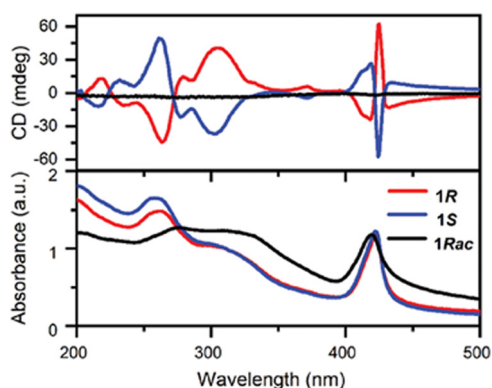
Fig. 21 CD spectra of (R/S\text{-}Rac\text{-}3AMP)\text{PbBr}_4 (above) along with their absorption spectra (below). Reprinted with permission from ref. 41 Copyright©2022 Wiley-VCH GmbH.
