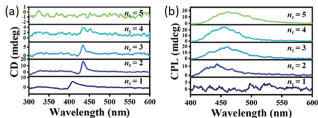
Fig. 28 (a) CD and (b) CPL spectra of (S/R\text{-}MBA)_2MA_{n-1}Pb_nBr_{3n+1} as a function of \langle n \rangle . Reprinted with permission from ref. 48 Copyright©2022 Wiley-VCH GmbH.
