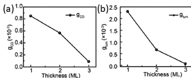
Fig. 29 (a) g_{CD} and (b) g_{CPL} of (S/R\text{-}MPA)_2Cs_{n-1}Pb_nBr_{3n+1} as a function of the layer thickness \langle n \rangle . Reprinted with permission from ref. 49 Copyright©2023 Wiley-VCH GmbH.
