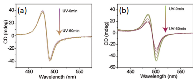
Fig. 10 CD spectra of (a) polymerized and (b) unpolymerized (S\text{-R-MBA})_2\text{PbI}_4 . Reprinted with permission from ref. 30 Copyright©2023 Wiley-VCH GmbH.
