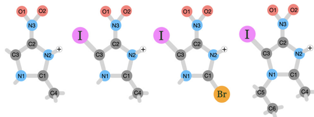
Fig. 1 Schematic picture of the studied protonated molecules. From left to right: \text{NimH}^+ , \text{INimH}^+ , \text{BrINimH}^+ , and \text{EtINimH}^+ .
