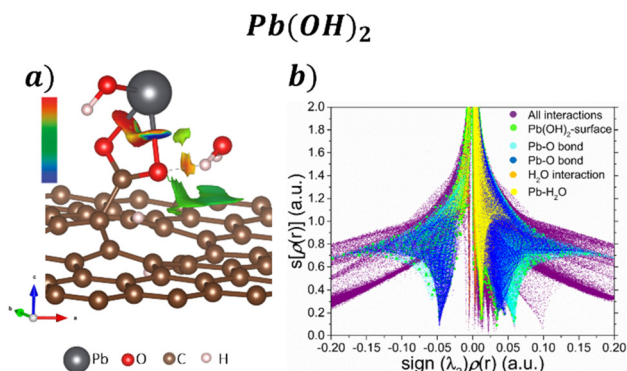
Fig. 6 a) NCI isosurface with s = 0.05 a.u. and b) s[\rho(r)] vs. \text{sign}(\lambda_2)\rho(r) graph for the adsorption Pb(OH) 2 on the GO surface.
