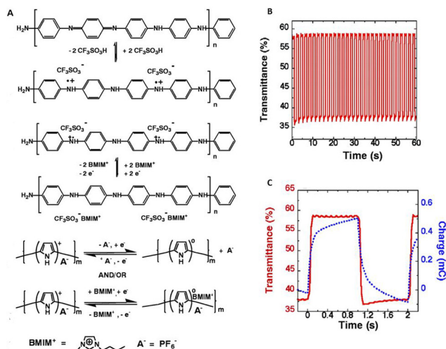
Fig. 6 (A) Electrochemical reactions of polyaniline and polypyrrole in the presence of ionic liquid; [\text{BMIM}]^+[\text{PF}_6]^- . (B) Demonstration of these polymers in electrochemical devices; the transmittance change obtained at 560 nm for a pixel of the same numeric display upon voltage switching between -1.5 V and +1.5 V with the pulse width of 1 s. (C) The charge versus time (dashed line) and \Delta T versus time (solid line) curves for a display pixel upon voltage switching between -1.5 and 1.5 V with a pulse width of 1 s. Reproduced from ref. 70 with permission from Science, Copyright [2002].
