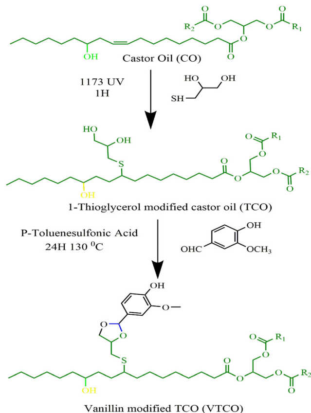
Scheme 1 Synthesis route of TCO and VTICO.
