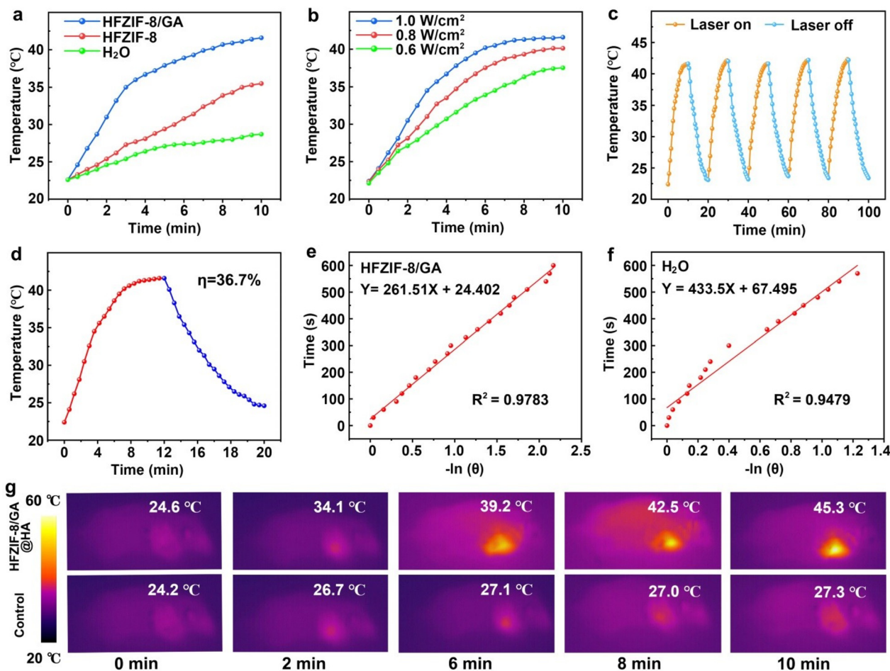
Fig. 3 Temperature changes of the HFZIF-8/GA degradation products, HFZIF-8, and H 2 O under 1064 nm laser irradiation (1064 nm, 1.0 W \text{cm}^{-2} ) for 10 min (pH 6.5) (a). Temperature change curves of HFZIF-8/GA's (500 \mu\text{g mL}^{-1} ) degradation products under irradiation for 10 min with different power intensities (pH 6.5) (b). Photothermal stability tests of HFZIF-8/GA (500 \mu\text{g mL}^{-1} ) under 1064 nm laser irradiation (1.0 W \text{cm}^{-2} ) after degradation (pH 6.5) (c). Heating-cooling cycles of HFZIF-8/GA (500 \mu\text{g mL}^{-1} ) after degradation in aqueous solution (d). Time versus the temperature negative natural logarithm in HFZIF-8/GA (e) and H 2 O (f) from the corresponding cooling tests, respectively. Thermal images of U14 tumor-bearing mice in different groups after 10 min NIR-II laser irradiation (g).
