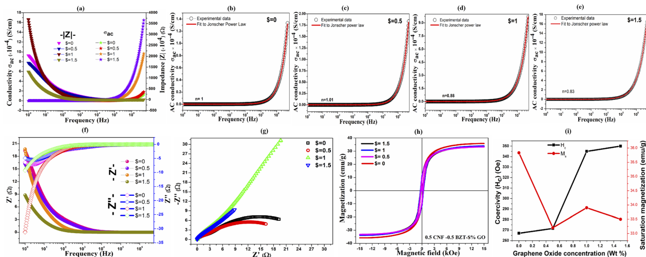
Fig. 6 (a) Conductivity and impedance as a function of frequency for GO decorated magnetoelectric composites. (b)–(e) Power law fitting curve for the AC conductivity of 0.5BZT–0.5CNF–$% GO ($ = 0, 0.5, 1, 1.5). (f) Bode plots. (g) Nyquist plot for composites. (h) Composite's magnetization curve as a function of magnetic field. (i) Variation in coercivity and saturation magnetization with GO content in the magnetoelectric composite.
