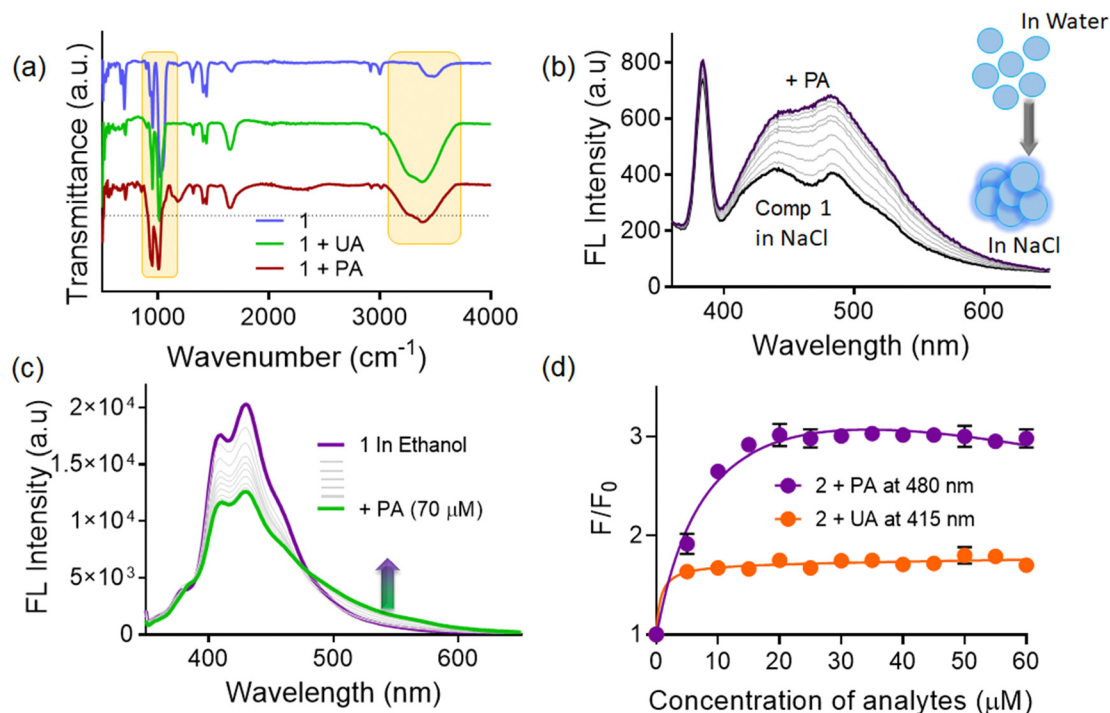
Fig. 5 (a) FTIR spectra of probe 1 in the presence of phytic acid and uric acid. (b) Fluorescence spectra of 1 (10 \mu M, \lambda_{\text{ex}} = 340 nm) upon phytic acid addition (0–70 \mu M) in 6.3 M NaCl. (c) Fluorescence spectra of 1 (10 \mu M, \lambda_{\text{ex}} = 340 nm) upon phytic acid addition (0–70 \mu M) in ethanol. (d) Fluorescence spectra of probe 2 (10 \mu M, \lambda_{\text{ex}} = 390 nm) upon phytic acid (0–60 \mu M) and uric acid (0–100 \mu M) addition in water.
