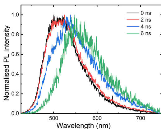
Fig. 4 Transient photoluminescence spectroscopy of a thin film of 1 (2 wt% in poly(styrene), \lambda_{\text{ex}} = 400 nm).
