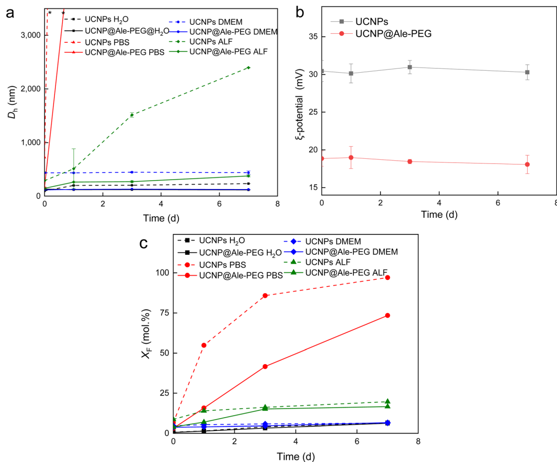
Fig. 5 Time dependencies of (a) hydrodynamic diameter D_h in water, PBS, DMEM and ALF, (b) \zeta -potential of UCNPs and UCNP@Ale-PEG nanoparticles in water and (c) F^- ion molar fraction ( X_F ) in the supernatants after incubation of particles in water, PBS (pH 7.4), DMEM and ALF at 37 °C. * Beyond the scope of measurement.
