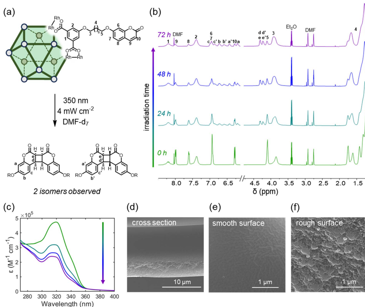
Fig. 3 (a) Irradiation of C 10 -Coumarin-RhMOP at 350 nm results in the dimerization of their side chains. (b) 1 H NMR spectra of a 5 mM DMF-d 7 solution of C 10 -Coumarin-RhMOP after irradiation at 350 nm for 0 h (green), 24 h (teal), 48 h (blue), and 72 h (purple) reveal the emergence two correlated sets of aromatic and alkyl signals, suggesting the formation of two coumarin dimer isomers. Note that the absolute stereochemical configurations of the dimer isomers corresponding to each set of correlated peaks cannot be verified by this technique, and are therefore assigned arbitrarily. (c) UV-Vis spectra of the MOP solution at each irradiation time point reveal a decrease in the coumarin \pi \rightarrow \pi^* peak at 320 nm, corroborating the formation of cyclobutane dimers. (d–f) SEM images of the (d) cross section, (e) smooth surface, and (f) rough surface of a photopolymerized C 10 -Coumarin-RhMOP thin film produced via 350 nm irradiation of a 20 mM DMF solution of the cage.
