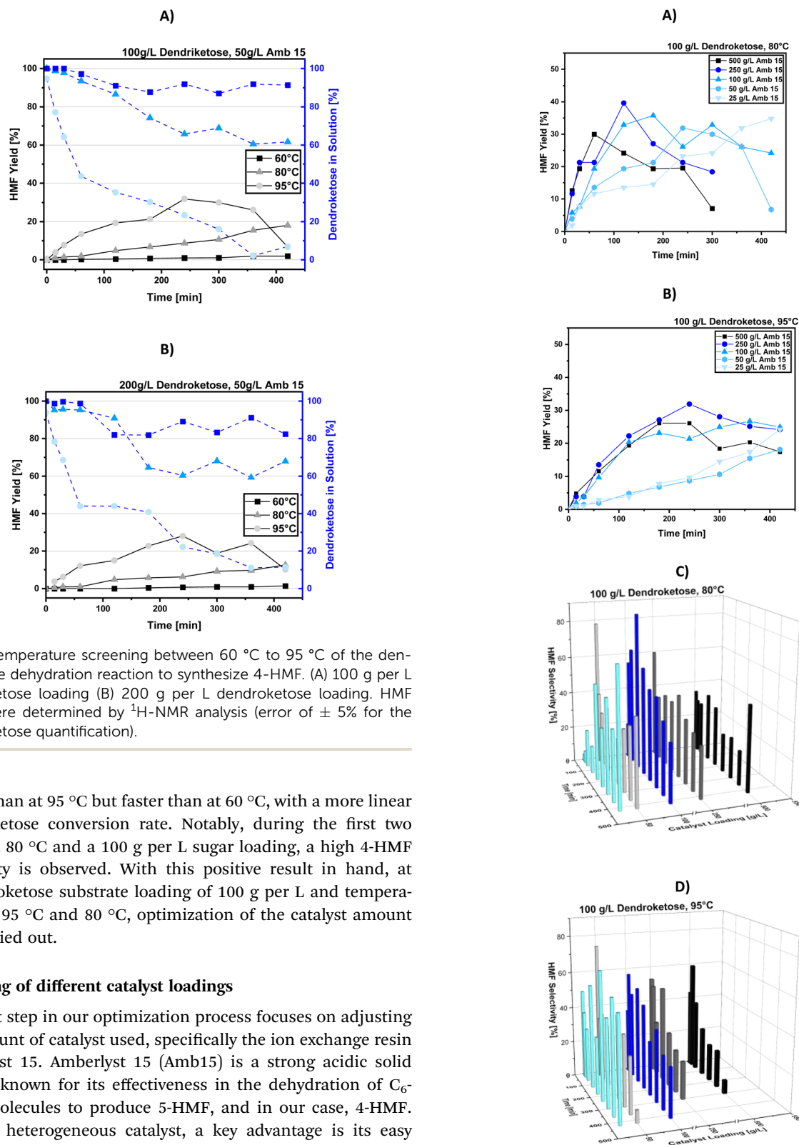
Fig. 6 Time resolved screening of the Amb15 catalyst loading between 10 g per L to 500 g per L for the dendroketose dehydration reaction to synthesize 4-HMF. (A) HMF yield at 100 g per L dendroketose loading and 80 °C, (B) HMF yield at 100 g per L dendroketose loading and 95 °C, (C) HMF reaction selectivity at 100 g per L dendroketose loading and 80 °C, (D) HMF reaction selectivity at 100 g per L dendroketose loading and 95 °C. HMF yields and selectivity were determined by ^1\text{H} -NMR analysis (error of \pm 5\% for the dendroketose quantification).
