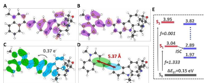
Figure 2 (A) HOMO; (B) LUMO; (C) electron-hole distribution for S_0 \rightarrow S_1 excitation process; (D) electron-hole separation; (E) energy level distribution of singlet and triplet states. Green and cyan surfaces represent electron and hole distributions, respectively; f represents the oscillator strength for the excitation process.
