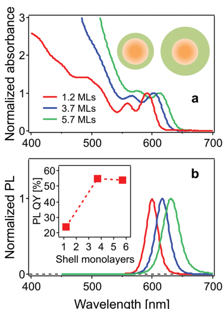
Fig. 1 (a) Normalized absorption and (b) PL spectra of CdSe/CdS QDs with 1.2, 3.7, and 5.7 monolayers of the CdS shell in chloroform. Inset in (a): a schematic diagram showing the CdSe/CdS core/shell structure with thin (left) and thick (right) shell. Inset in (b): the PL quantum yield as a function of CdS shell thickness.
