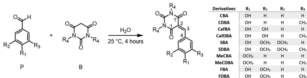
Scheme 1 Synthesis of phenolic barbituric acid derivatives synthesis: coumaryl barbituric acid (CBA), coumaryl dimethyl barbituric acid (CDBA), caffeyl barbituric acid (CafBA), caffeyl dimethyl barbituric acid (CafDBA), sinapyl barbituric acid (SBA), sinapyl dimethyl barbituric acid (SDBA), 4-methoxy coumaryl barbituric acid (MeCBA), 4-methoxy coumaryl dimethyl barbituric acid (MeCDBA), ferulyl barbituric acid (FBA), and ferulyl dimethyl barbituric acid (FDDBA). The central C atoms in the product are labelled consistently with the numbering scheme used in the electronic structure calculations.
