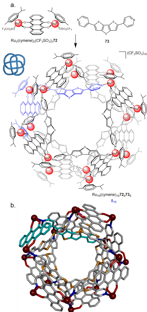
Fig. 25 (a) Synthesis of 8_{18} metalla-knot \text{Ru}_{16}(\text{p-cymene})_{16} \mathbf{72} \mathbf{73}_8 . (b) X-ray crystal structure of the 8_{18} metalla-knot with p -cymene ligands omitted for clarity. 100
