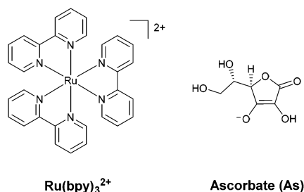
Fig. 1 The molecular structures of the Ru(bpy) 3 2+ photosensitizer and the ascorbate sacrificial electron donor used in combination with cobalt polypyridine complexes for light-driven hydrogen evolution studies.
