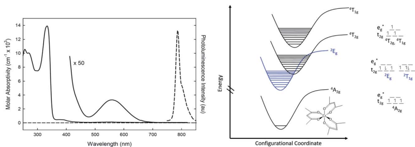
Fig. 8 (Left) Solution-phase absorption (solid line) and 90 K emission (dashed) spectra of Cr(acac) 3 . The broad absorption centered at 560 nm corresponds to the lowest energy 4 A 2 → 4 T 2 ligand-field absorption, whereas the emission at 790 nm arises from the 2 E excited state that is formed in <100 fs following excitation. Adapted from ref. 23. (Right) Qualitative potential energy surface diagrams appropriate for Cr(acac) 3 , with the corresponding ligand-field splitting diagrams depicting the valence d-orbital based electronic structure. The PES for the 2 T 1g state has been omitted for clarity.
