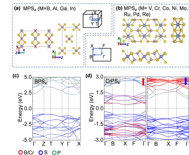
Fig. 5 (a) and (b) Atomic structures of assembled bulk MPS 4 (M = B, Al, Ga, In) and an MPS 4 (M = V, Cr, Co, Ni, Mo, Ru, Pd, and Re) monolayer, respectively, displayed from different perspectives. The M, P, and S atoms are shown in blue (pink), purple, and yellow colors, respectively. The corresponding Brillouin zones are illustrated. (c) and (d) Electronic band structures of assembled bulk BPS 4 and monolayer CrPS 4 , respectively. The contributions from different atoms or orbitals are shown by color. The Fermi level is shifted to zero (dashed lines).
