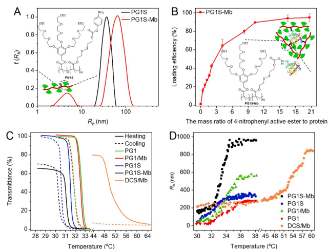
Fig. 2 (A) Plots of R_h from PG1S and PG1S-Mb. 25 °C, C = 0.05 \text{ mg mL}^{-1} . The size polydispersities were 0.40 and 0.59, respectively. (B) Loading efficiency of PG1S for Mb at different concentrations. (C) Plots of transmittance vs. temperature for PG1S, PG1S-Mb, PG1, PG1/Mb, and DCS/Mb. C = 2.5 \text{ mg mL}^{-1} . (D) Plots of R_h for PG1S, PG1S-Mb, PG1, PG1/Mb, and DCS/Mb between 30 and 60 °C, respectively. C = 0.05 \text{ mg mL}^{-1} .
