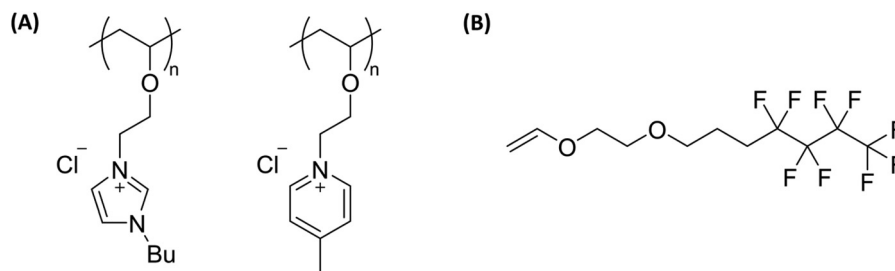
Fig. 30 Chemical structure of (A) poly[2-(vinyl-oxo)-ethyl-1-butylimidazolium chloride] and poly[2-(vinyl-oxo)-ethyl-4-methylpyridinium chloride], 155 and (B) the 2-(4,4,5,5,6,6,7,7,7-nonafluoroheptyloxy)ethyl vinyl ether (9FVE) partially fluorinated monomer. 153
