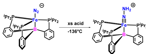
Fig. 31 Fe \equiv N-NH_2 Intermediate for catalytic Reduction of N_2 .
