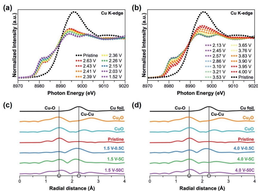
Fig. 4 XAS of [\text{CuL(Py)}_2]_n electrodes: (a) and (b) in situ Cu K-edge XANES patterns during discharge and charge at 20 \text{ mA g}^{-1} ( \sim 0.08\text{C} ), respectively. (c) and (d) Ex situ Cu K-edge EXAFS patterns at three different rates (0.5C, 5C and 50C) at end of discharge (1.5 V) and end of charge (4.0 V), respectively (with Cu foil, \text{Cu}_2\text{O} and CuO as references).
