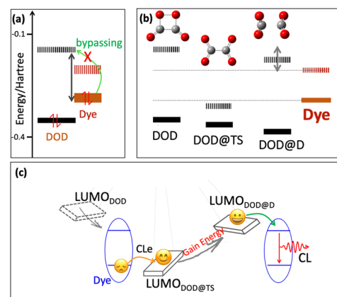
Fig. 3 Electronic properties of the CL system. (a) The relative HOMO and LUMO energy levels of the DOD and cyanine dyes. (b) The relative HOMO and LUMO energy levels of the DOD, \text{DOD@TS} (Transition State), \text{DOD@D} (Dissociated state) and cyanine dyes. (c) Orbital swing scheme for the electron transfer of the single-dye NIR-II CL system.
