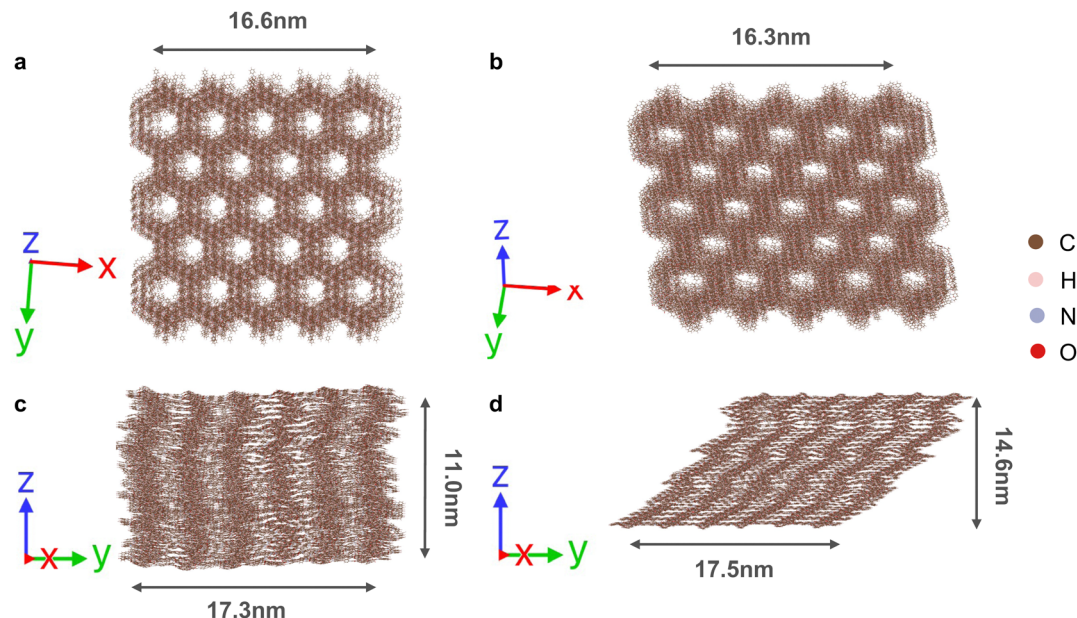
Fig. 9 Snapshots of the supercells of (a and c) zagzig Tp-Azo, (b and d) inclined Tp-Azo at equilibrium from classical force field calculations. The scale size of each snapshot of a, b and c are labelled. The viewed direction of each snapshot is indicated at the bottom left.
