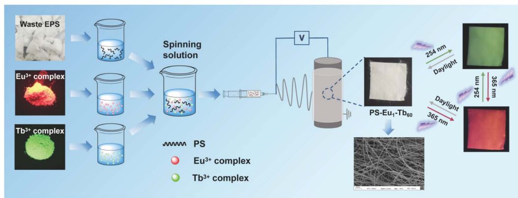
Fig. 1 Fabrication illustration of the UV-excited dual-mode luminescent electrospun fiber membranes from waste EPS.
