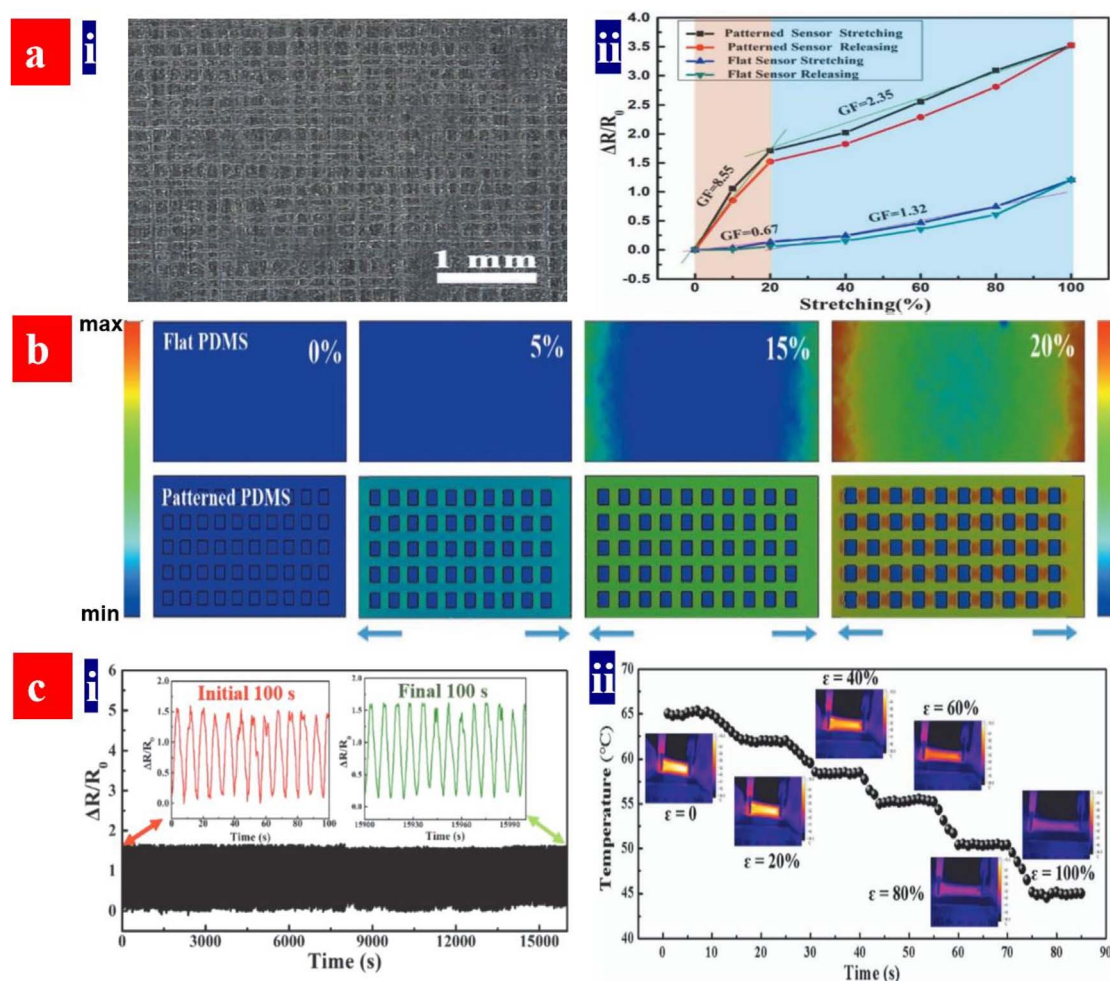
Fig. 17 (a) (i) Optical micrograph of the polyacrylonitrile grids fabricated by near-field electrospinning with a spacing distance ( d ) of 150\text{ }\mu\text{m} , and (ii) relative resistance changes versus tensile strains of the strain sensors based on the flat and patterned electrodes. (b) Stress distributions of both flat- and patterned PDMS substrates with d = 150\text{ }\mu\text{m} during the first straining process. (c) (i) Relative resistance changes versus times (1–16000 s) of the sensors under \varepsilon = 20\% , and (ii) temperature changes versus strains for the strain sensors. Reproduced with permission. 193 Copyright 2020, Wiley-VCH.
