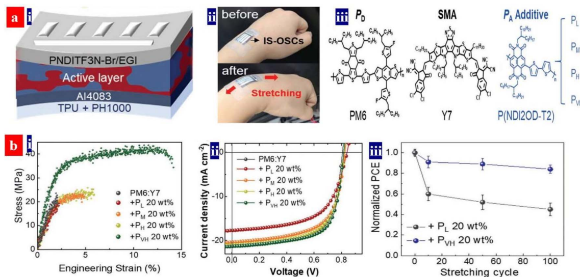
Fig. 20 (a) (i) Stretchable OSC structure, (ii) photographs, and (iii) molecular structures of the PA additives. (b) (i) Stress–strain curves of PM6:Y7 with 20 wt% of PAs of different M_w s, (ii) J–V curves of the stretchable OSCs as functions of PAs with different M_w s, and (iii) normalized PCE curves of the stretchable devices in the flexing tests. Reproduced with permission. 199 Copyright 2022, Wiley-VCH.
