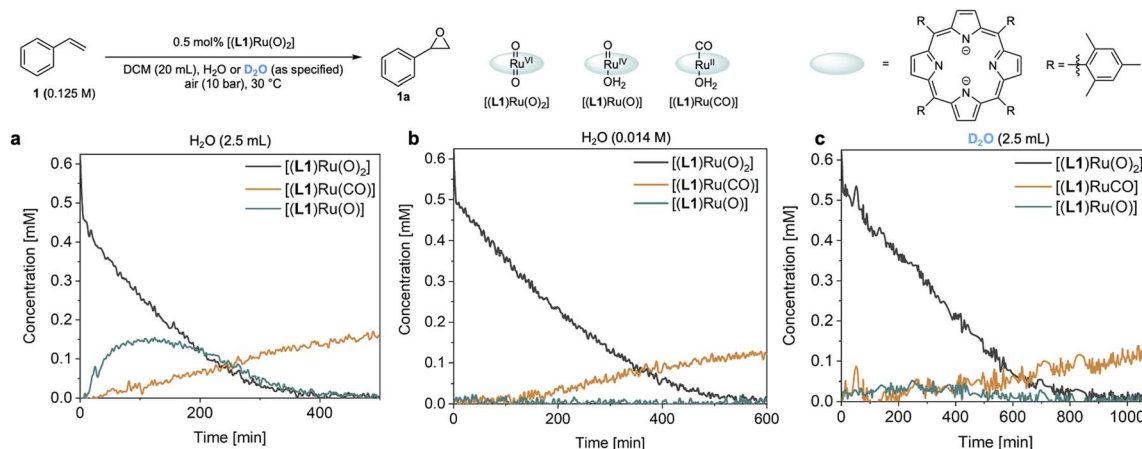
Fig. 4 Operando catalyst speciation studies. (a) Distribution of ruthenium species observed by ^1H FlowNMR spectroscopy in DCM saturated with an excess of H_2O . (b) Distribution of ruthenium species observed by ^1H FlowNMR spectroscopy in laboratory grade DCM (14 mM). (c) Distribution of ruthenium species observed by ^1H FlowNMR spectroscopy in DCM saturated with an excess of D_2O (99.9% atom% D).
