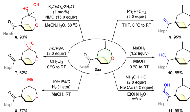
Scheme 4 Synthetic transformations.
