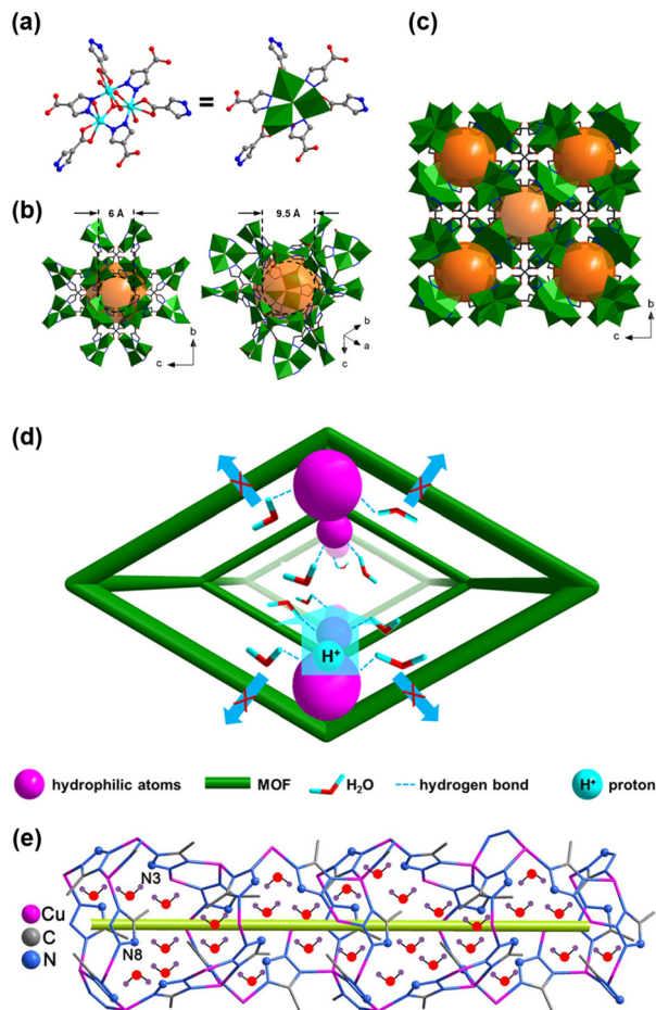
Fig. 5 Schematic diagrams of CuCpz. (a) Cu 3 (μ 3 -OH) clusters in CuCpz; (b) accessible window apertures of the cage structure; and (c) unit cell. All NH 4 + ions in the pore and the hydrogen atoms of the ligands are omitted for clarification. The Cu, O, N, and C are shown in cyan, red, blue, and gray, respectively. (d) Proposed holding effect scheme of the hydrophilic atoms in the CuCpz pores for enhancing the proton conductivity at reduced RH. Reproduced with permission from ref. 59, Copyright 2022, American Chemical Society. (e) Tunnel in the 3D anionic [Cu 3 (mtz) 4 ] − framework of 1 with schematic guest water molecules. Red and purple balls present O and H atoms, respectively. The green, yellow bar highlights the proton pathway. Reproduced with permission from ref. 64, Copyright 2021, American Chemical Society.
