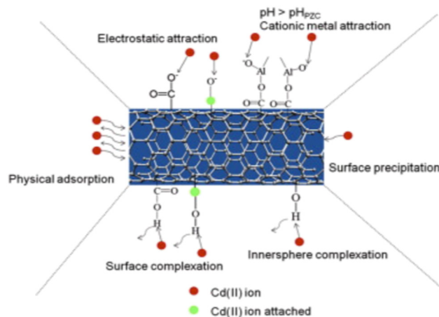
Fig. 4 Schematic showing the interaction of \text{Cd(II)} ions with \text{Al}_2\text{O}_3/\text{MWCNTs} . 30
