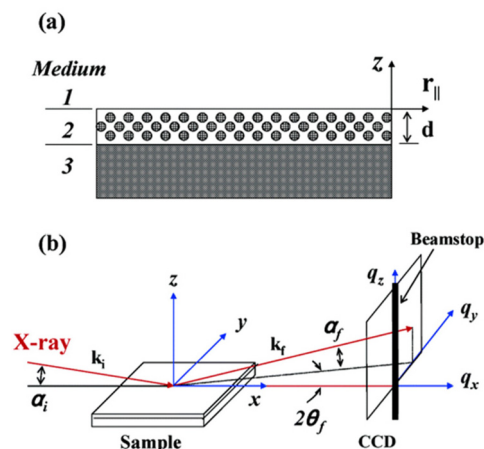
Fig. 10 General GI-SAXS setup: (a) medium 1 = vacuum; medium 2 = mesostructured thin film with thickness d ; medium 3 = substrate with infinite thickness. (b) \alpha_i = incident angle; \alpha_f and 2\theta_f = exit angles of the X-ray beam. k_i and k_f = wave vector of the incident and scattered X-ray beams. q_x , q_y , and q_z = components of the scattering vector q . Reproduced from ref. 142 with permission from ACS, copyright 2025.
