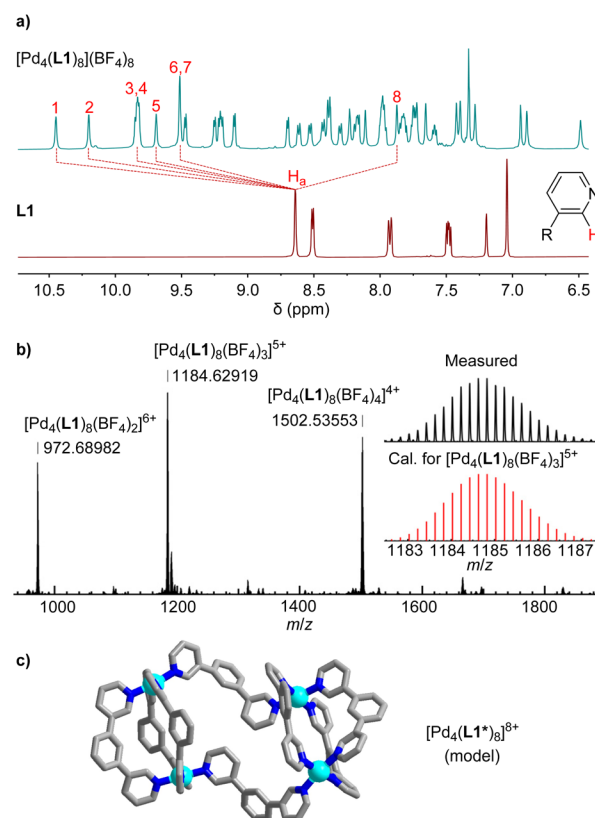
Fig. 2 (a) 1 H NMR spectra (400 MHz, D 2 O) of [Pd 4 ( L1 ) 8 ](BF 4 ) 8 and of ligand L1 . (b) High resolution ESI mass spectrum of [Pd 4 ( L1 ) 8 ](BF 4 ) 8 . (c) Molecular model of [Pd 4 ( L1 *) 8 ] 8+ (the side chains were omitted).
