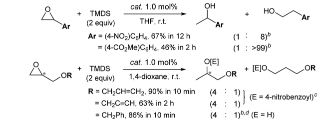
Scheme 5 Substrate scope of the Piers' borane-catalysed hydrosilylation. a Yields were determined using 1 H NMR. b The desired alcohol products were isolated upon hydrolysis with saturated K_2CO_3 in MeOH. c The crude products were O -benzoylated in situ through the reaction with 4-nitrobenzoyl chloride. d ( S )-1-(Benzyloxy)propan-2-ol was obtained as a major product with >98% ee.
