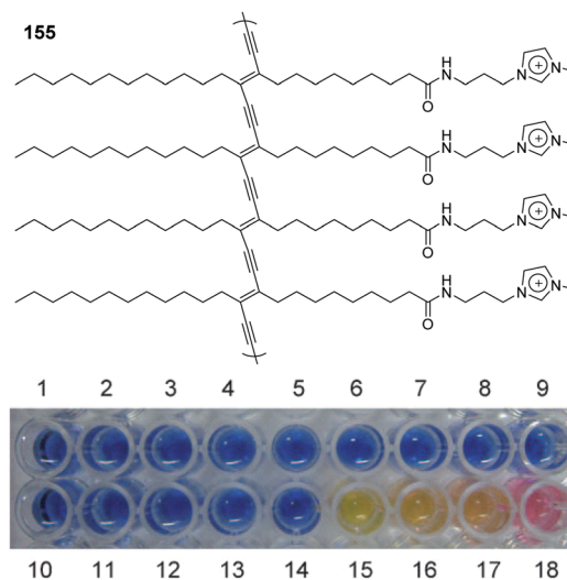
Fig. 14 Structure of polymerized 155 , and colorimetric responses of polymerized 155 (100 nm) in the presence of various analytes (500 \mu m) in HEPES buffer (20 mM, pH 7.4): 1 blank, 2 F − , 3 Cl − , 4 Br − , 5 I − , 6 SO 4 2− , 7 CO 3 2− , 8 ClO 4 − , 9 CH 3 COO − , 10 NO 3 − , 11 HPO 4 2− , 12 SCN − , 13 CTAC, 14 Triton X-100, 15 SDS, 16 SDC, 17 SDP, 18 SDBS.
