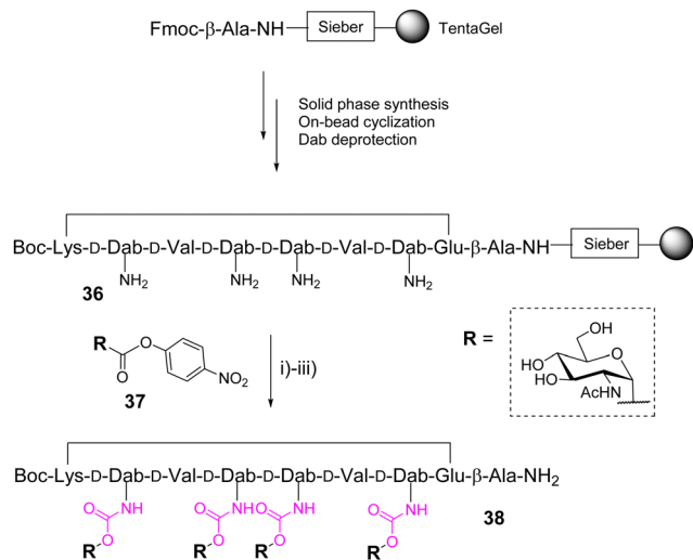
Scheme 6 On-bead synthesis of a glycosyl carbamate-cyclopeptide 38 using glycosyl p -nitrophenyl carbonate 37 . Reagent and conditions: 37 , DIPEA, NMP; (ii) TFA/TIS/ \text{CH}_2\text{Cl}_2 (1 : 1:98); (iii) NaOMe, MeOH/ \text{CHCl}_3 , 15%. Abbreviations: DIPEA: diisopropylethylamine; NMP: N -methylmorpholine.
