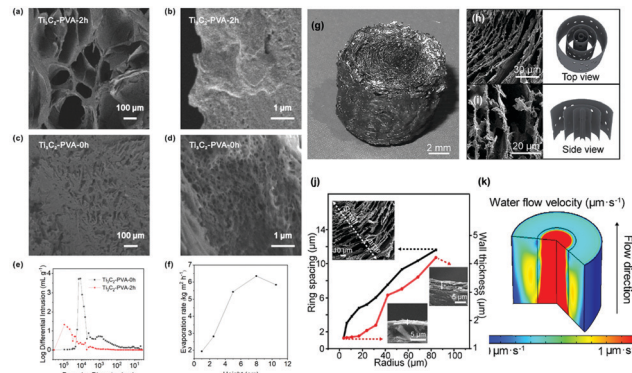
Fig. 10 (a–d) SEM images of \text{Ti}_3\text{C}_2\text{-PVA-2 h} and \text{Ti}_3\text{C}_2\text{-PVA-0 h} . (e) Pore size distribution. (f) The evaporation rates and the corresponding maximum water transport height. Reproduced with permission. 53 Copyright 2020, American Chemical Society. (g) Photo of the N-RGO aerogel with a ring-like architecture. The SEM images and corresponding schemes from (h) the top and (i) side views. (j) From the middle to the edge, the wall thickness and spacing increase. (k) Simulation of the ring-like aerogel's water flow velocity with gradient microchannels, suggesting concentrated pumping in the middle. Reproduced with permission. 116 Copyright 2020, American Chemical Society.
