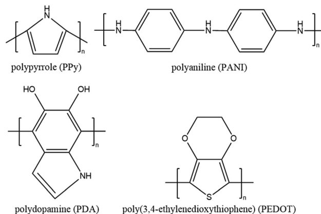
Fig. 4 Chemical structures of PPy, PANI, PDA and PEDOT with \pi -conjugated backbones of sp^2 -hybridized carbon.
