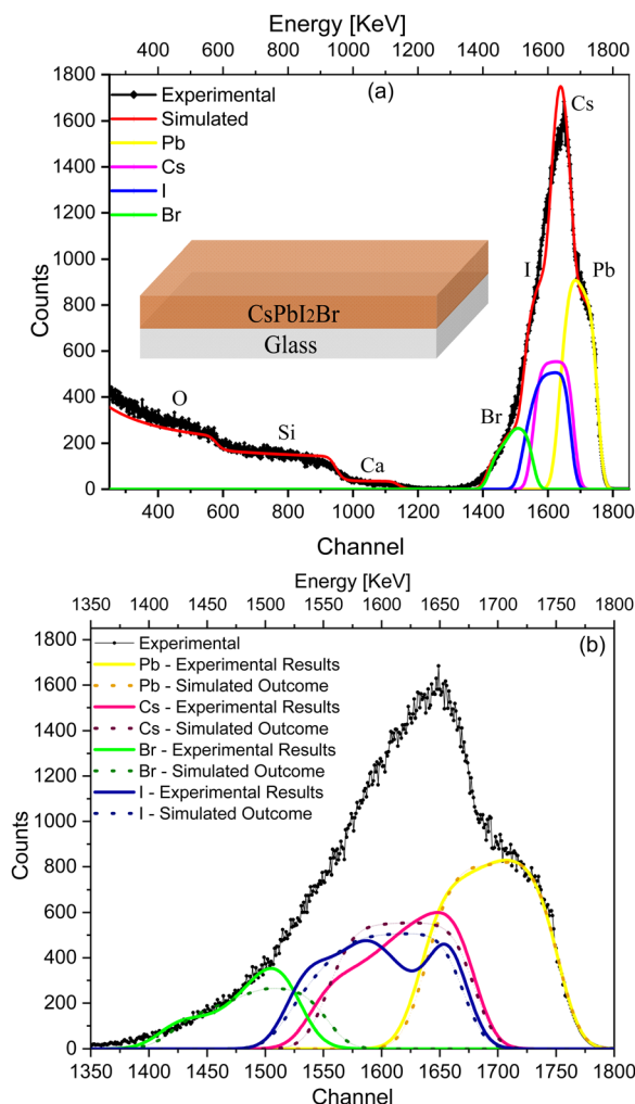
Fig. 2 (a) Simulated envelope of RBS in comparison with the experimental data for IHP ( \text{CsPbI}_2\text{Br} ) deposited on glass. (b) Comparison of the elemental (I, Br, Cs, and Pb) spectra of the simulated envelope (dotted lines) and the experimental fitting envelope (solid lines).
