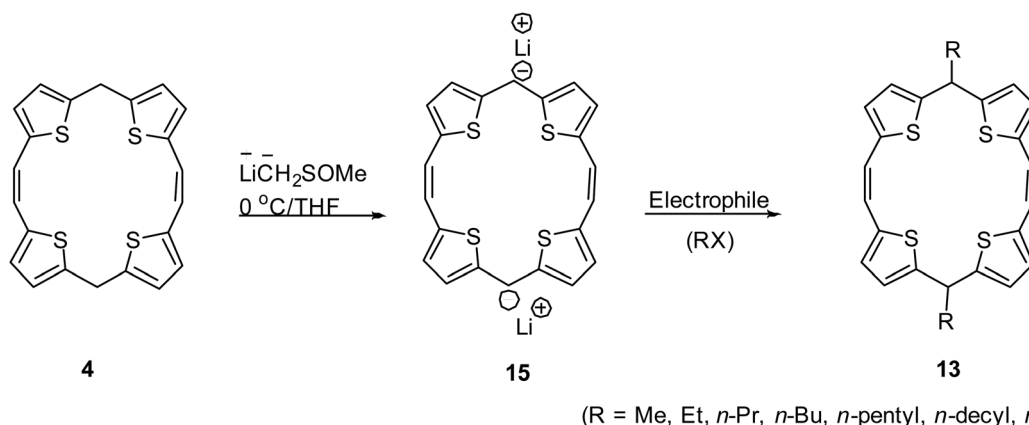
Scheme 4 Regioselective lithiation-substitution protocol for the direct synthesis of 5,16-dihydro TTPs.
