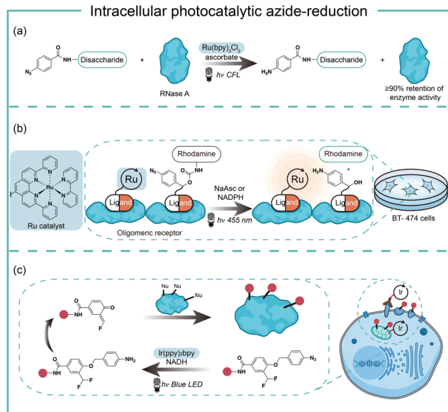
Fig. 8 Intracellular photocatalytic azide-reduction via visible-light irradiation. (a) The biomolecule-compatible photocatalytic azide-reduction by the Ru catalyst. (b) The photocatalytic decaging of azides by the Ru catalyst for in vivo fluorophore release. (c) The photocatalytic decaging of azides by the Ir catalyst for in vivo protein labeling.
