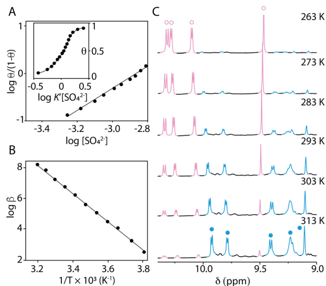
Fig. 4 (A) Hill plot obtained from a titration of SO 4 2- into a CD 3 OD solution of the Solomon link at 313 K. The insert shows the corresponding speciation curve. 34 In this plot, [SO 4 2- ] is normalized by the apparent equilibrium constant K' corresponding to the concentration of SO 4 2- producing half-occupation. (B) Van't Hoff plot. (C) Variable temperature 1 H NMR spectra of the Solomon link after addition of 2.6 equiv. of sulfate (CD 3 OD, 500 MHz). The signals corresponding to conformers 1 and 2 are coloured in pink (○) and blue (●), respectively.
