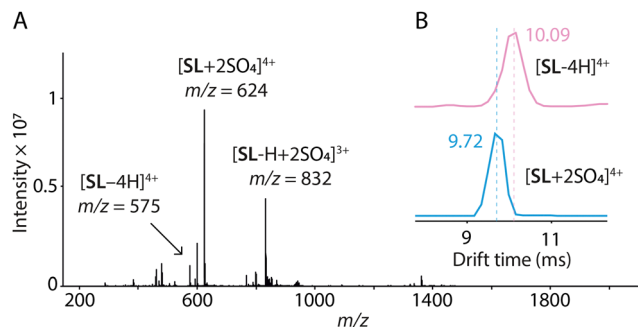
Fig. 3 (A) (+)ESI-MS spectrum of the Solomon link after addition of sulfate (1:1 molar ratio, 1 \mu M each) in CH 3 OH. (B) Representation of the ion-mobility mass spectrometry drift times and arrival time distributions at m/z 575 and 624, corresponding to ions [SL-4H] 4+ (in pink) and [SL + 2SO 4 ] 4+ (in blue), respectively.
