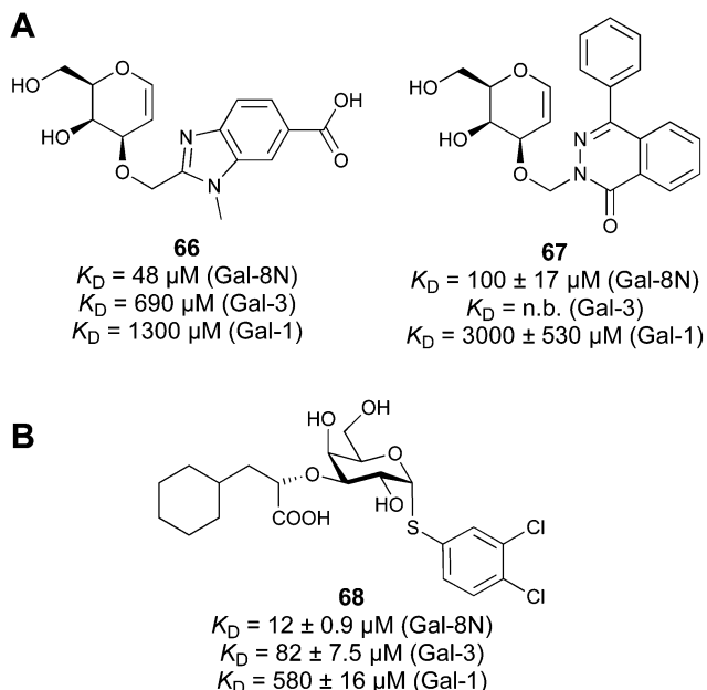
Fig. 13 Gal-8N inhibitors and their binding affinities for Gal-8N, Gal-3 and Gal-1, highlighting the selectivity for Gal-8N. (A) D-Galactals, (B) 3-lactoyl- \alpha -D-thiogalactopyranoside. n.b. = no binding.
