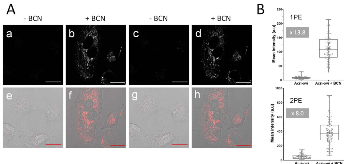
Fig. 7 (A) Confocal microscopy imaging of live A549 cells incubated with Acrid-oxyl at 2 \mu\text{M} for 3 h and then with (b and d) or without (a and c) BCN at 50 \mu\text{M} for 30 min under one (496 nm, a and b) or two-photon excitation (840 nm, c and d). (e), (f), (g) and (h) The corresponding merged images (fluorescence and brightfield). Emission slit settings: 500–700 nm. Scale bar: 20 \mu\text{m} . (B) Fluorescence quantification in live A549 cells with Acrid-oxyl (2 \mu\text{M} ) and BCN (10 \mu\text{M} ). Box plot represents the fluorescence intensity obtained by measuring pixel means using ImageJ software under one (1PE) (up) or two-photon excitation (2PE) (down). Data come from three independent experiments, and settings and processing were identical for all images. **** p < 0.0001 .
