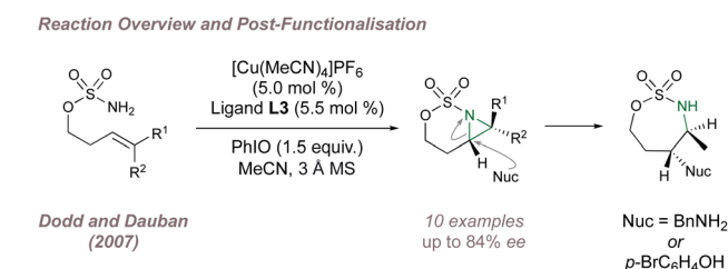
Fig. 3 Dodd and Dauban's enantioselective intramolecular aziridination of aliphatic alkenes.
