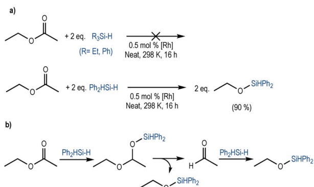
Scheme 1 (a) Reaction of ethyl acetate (0.25 mmol) with hydrosilanes (0.5 mmol) using a [Rh(SiS t Bu)] complex (0.5 mol%) at 298 K (neat, 16 h). Yields were calculated based on 1 H NMR (CDCl 3 ) analysis using 1,2-dichloroethane (0.0625 mmol) as an internal standard. (b) Proposed reaction pathways for the reduction of ethyl acetate using Ph 2 SiH 2 .
